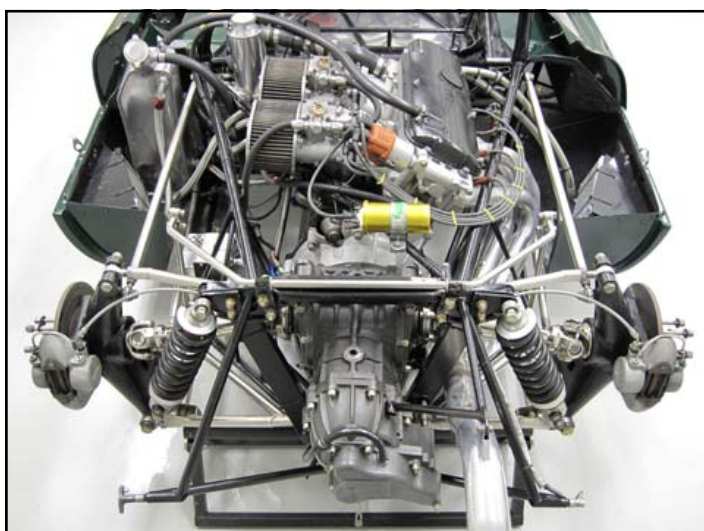
Rear Close Up Body Off
